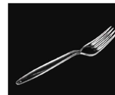
100 Fork weight: 5.03g size: 178x26.47x18.1mm material: GPPS
